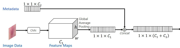
(a) Conventional concatenation-based data fusion
